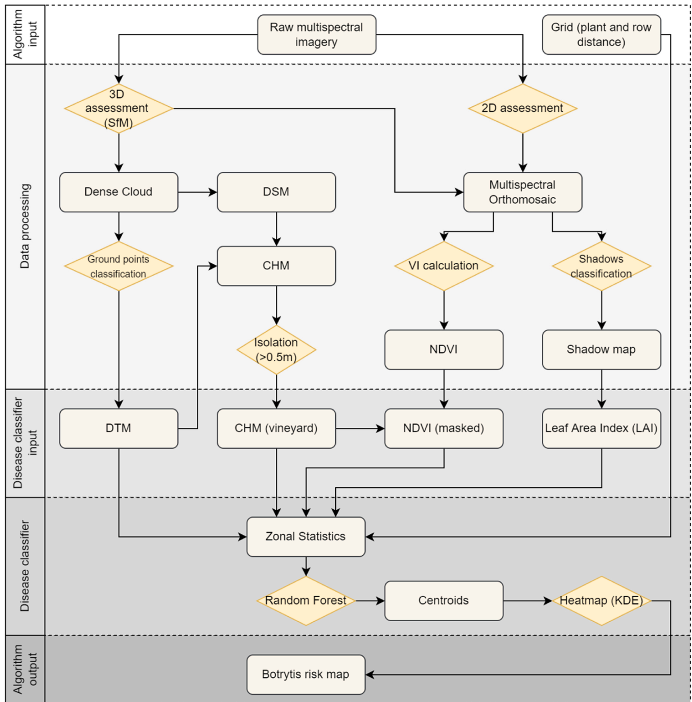
Fig. 4. – Workflow of the proposed methodology to obtain the Botrytis risk map. The initial inputs are the raw multispectral images and the grid defined by the distance between plants and rows. The inputs for the disease classifier are the DTM (Digital Terrain Model), CHM (Canopy Height Model), NDVI (Normalized Difference Vegetation Index) and LAI (Leaf Area Index). Finally, the Botrytis risk map is the predicted heatmap computed using Random Forest and kernel density estimation.
