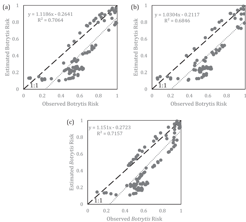
Fig. 10. Botrytis risk estimated vs predicted correlations according to heatmaps. Sample points: (a) Plants (b) Botrytis ground-truth points (c) Random Points within the ROI. Significance level: p\text{-value} < 0.05 .
